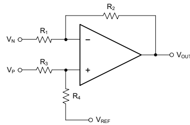
Figure 2. Difference Amplifier
