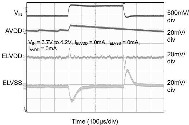
Line Transient No Load
