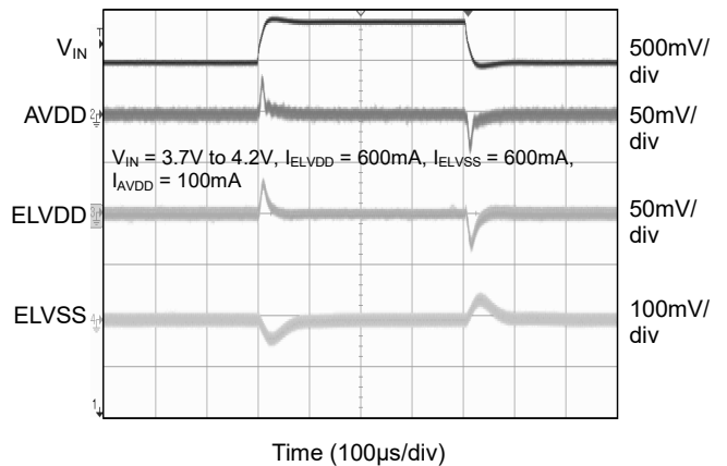
Line Transient Heavy Load
