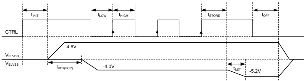
Figure 3. SGM3836D Programming V ELSS
