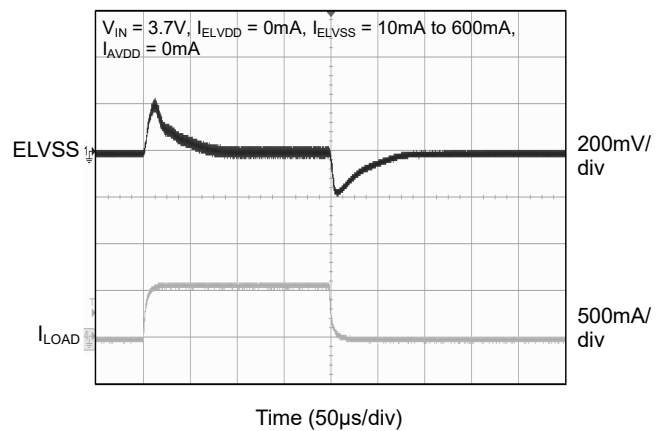
ELVSS Load Transient
