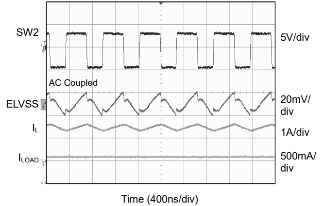
Output Ripple, ELVSS = -4.0V/600mA Load
