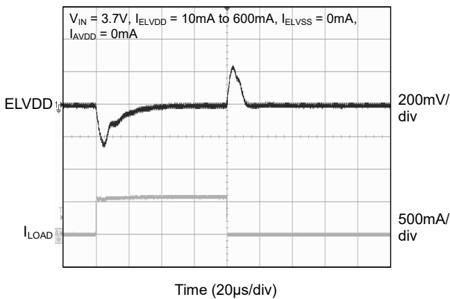
ELVDD Load Transient
