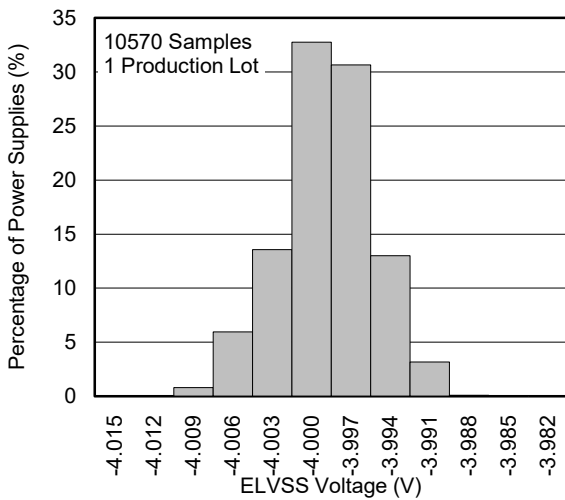
ELVSS (-4.0V) Voltage Production Distribution
