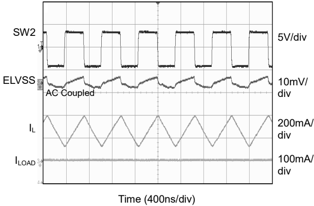
Output Ripple, ELVSS = -4.0V/100mA Load
