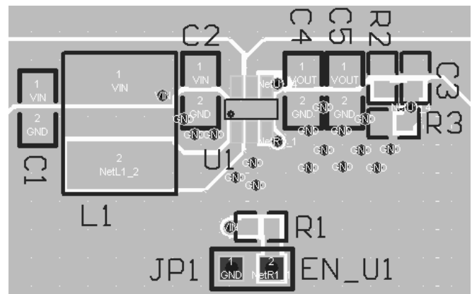
Figure 5. Layout Example
