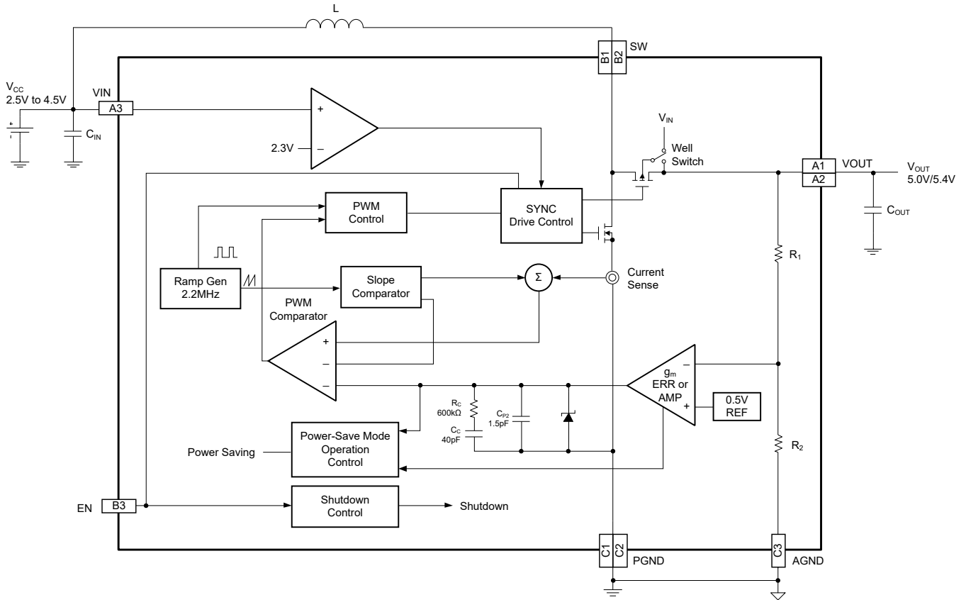
Figure 2. Block Diagram
